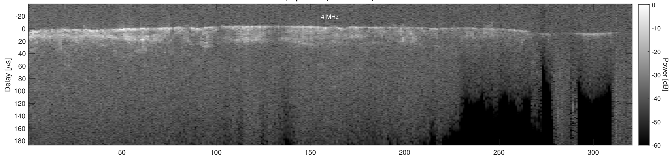
Orbit 4387, Cluttergram
