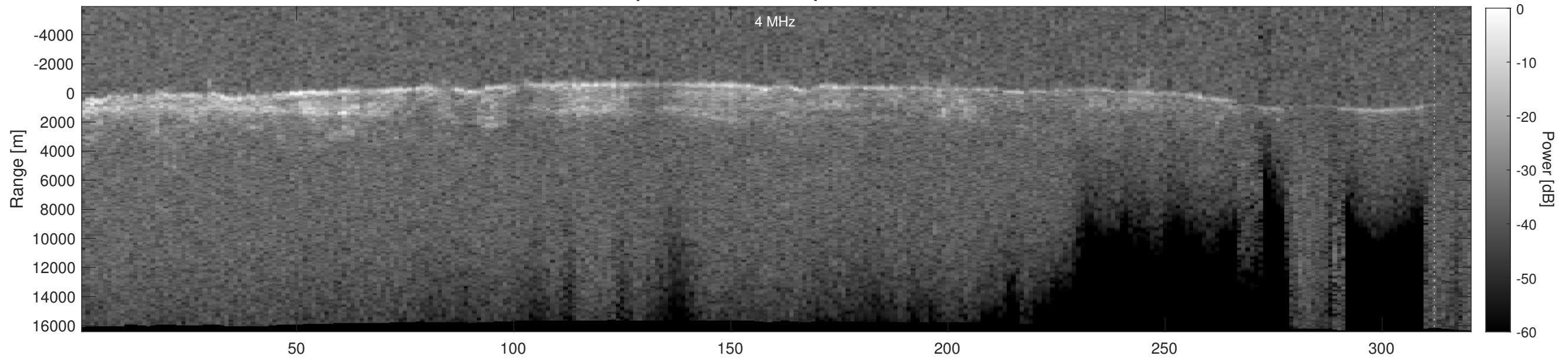
Orbit 4387, Depth-Corrected Cluttergram
