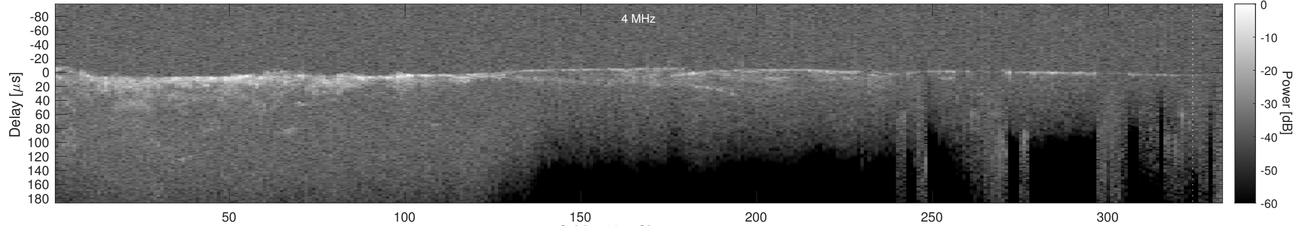
Orbit 4391, Cluttergram
