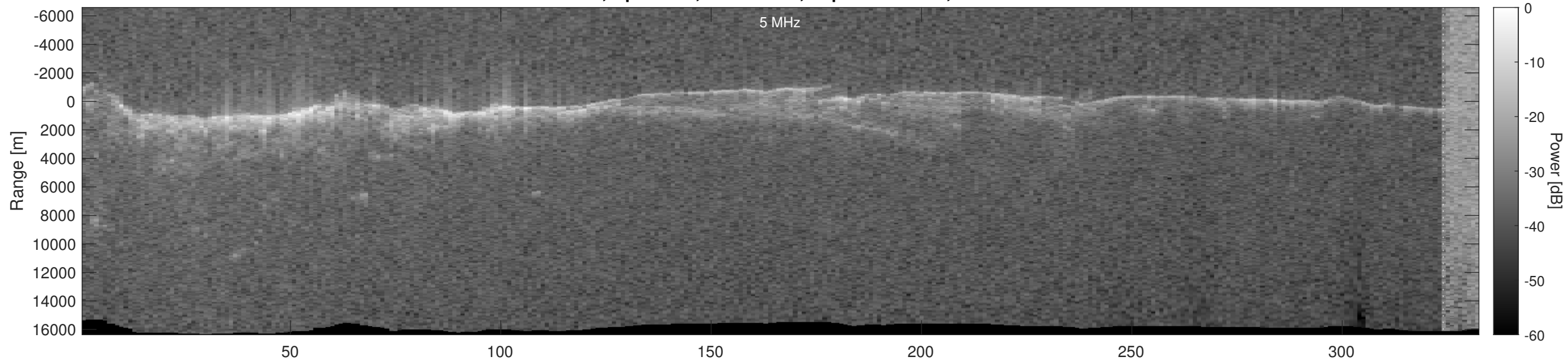
Orbit 4391, Optimized, No Window, Depth-Corrected, Channel 2
