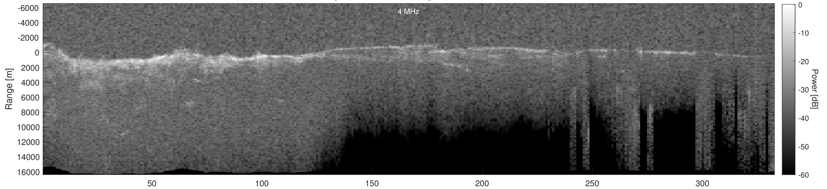
Orbit 4391, Depth-Corrected Cluttergram
