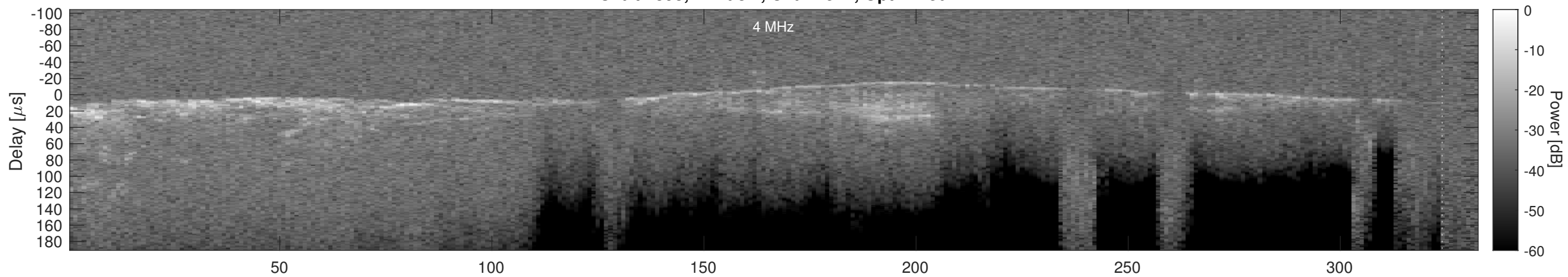
Orbit 4393, Cluttergram
