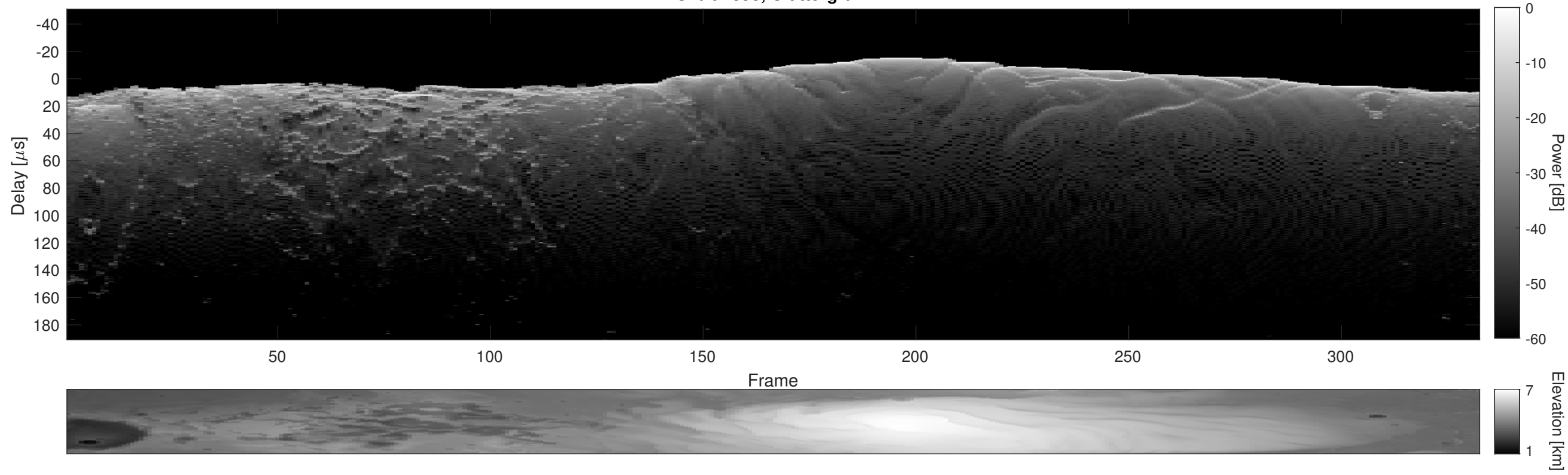
Orbit 4393, Cluttergram
