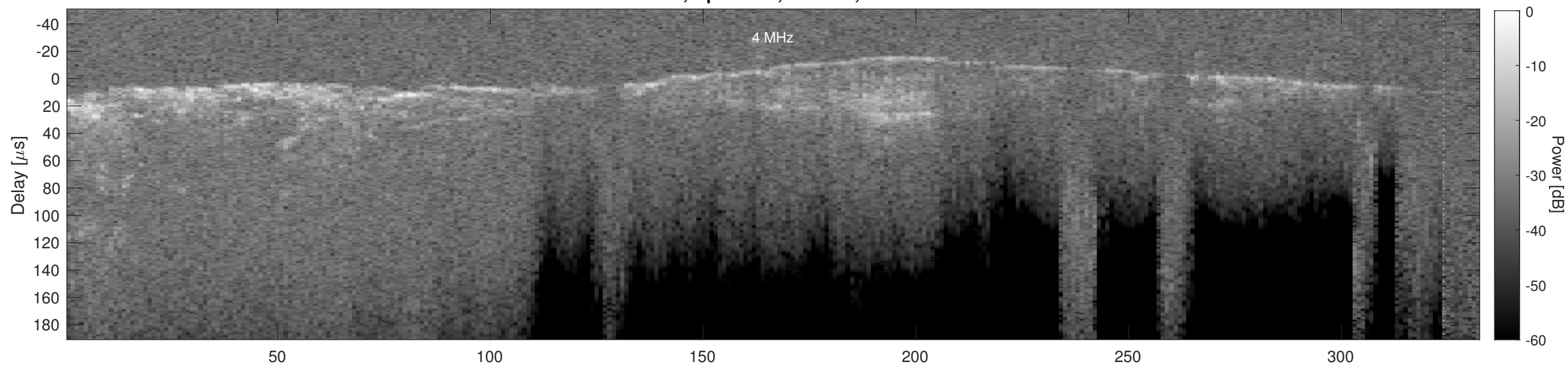
Orbit 4393, Cluttergram
