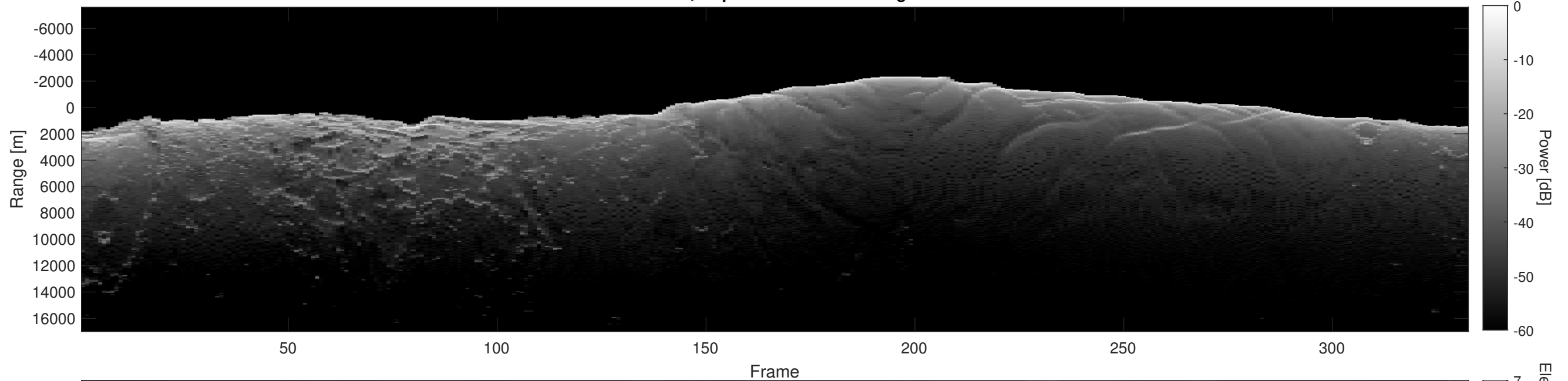
Orbit 4393, Depth-Corrected Cluttergram
