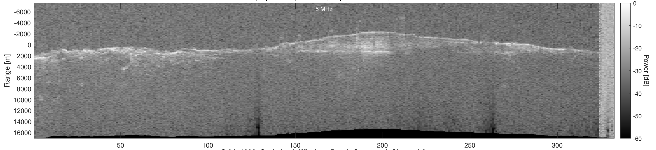
Orbit 4393, Optimized, Window, Depth-Corrected, Channel 2
