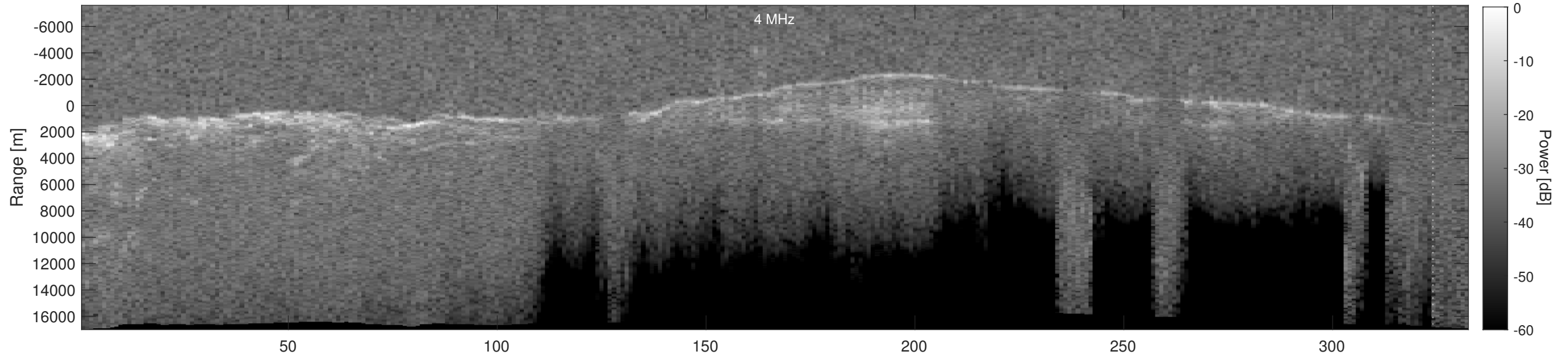
Orbit 4393, Depth-Corrected Cluttergram
