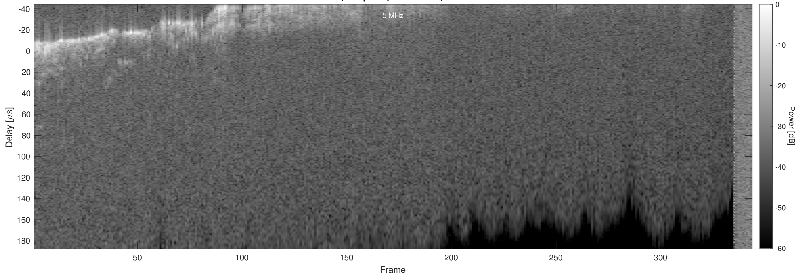
Orbit 4394, Chapman, No Window, Channel 2
