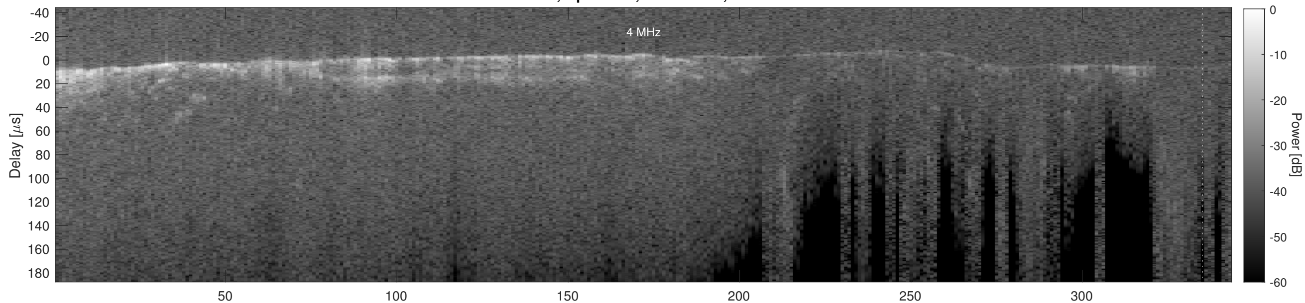
Orbit 4394, Cluttergram
