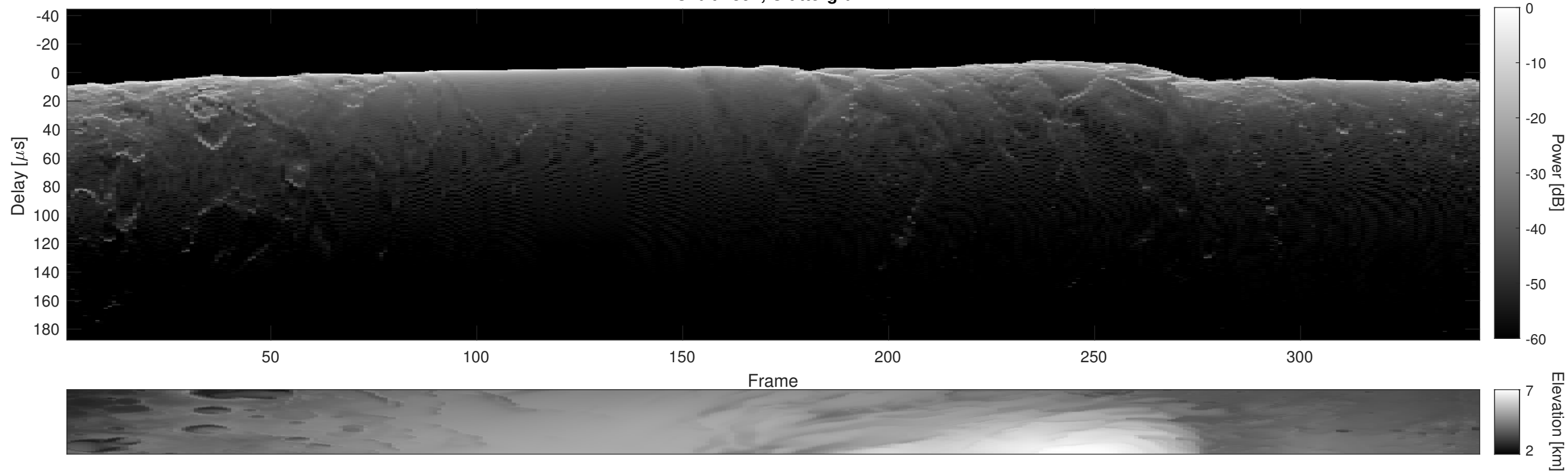
Orbit 4394, Cluttergram
