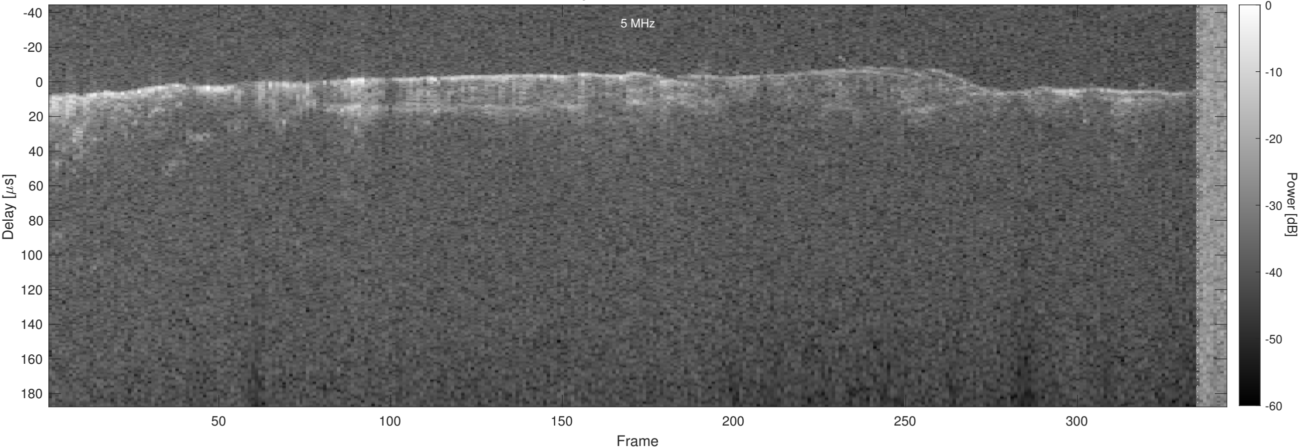
Orbit 4394, Optimized, Window, Channel 2
