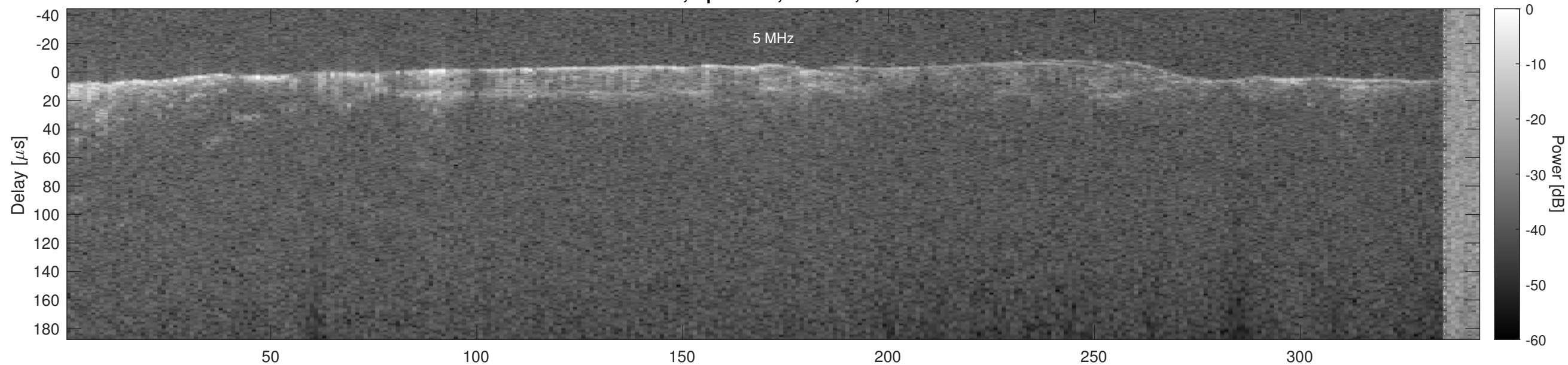
Orbit 4394, Optimized, Window, Channel 2
