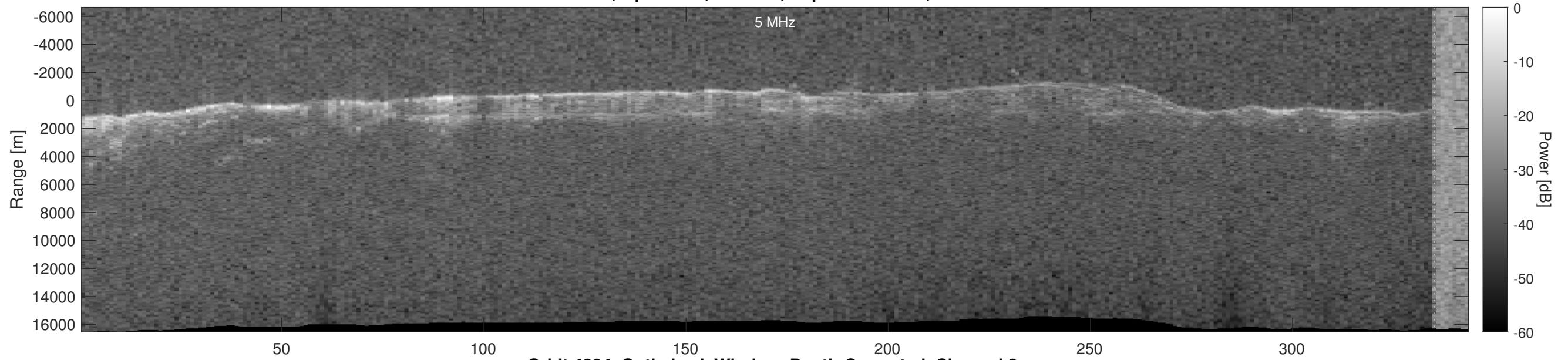
Orbit 4394, Optimized, Window, Depth-Corrected, Channel 2
