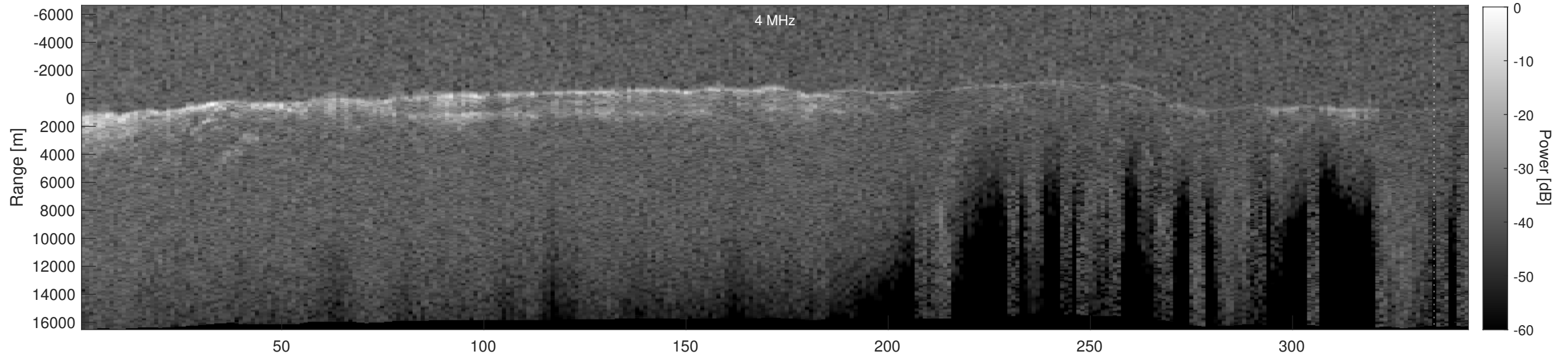
Orbit 4394, Depth-Corrected Cluttergram
