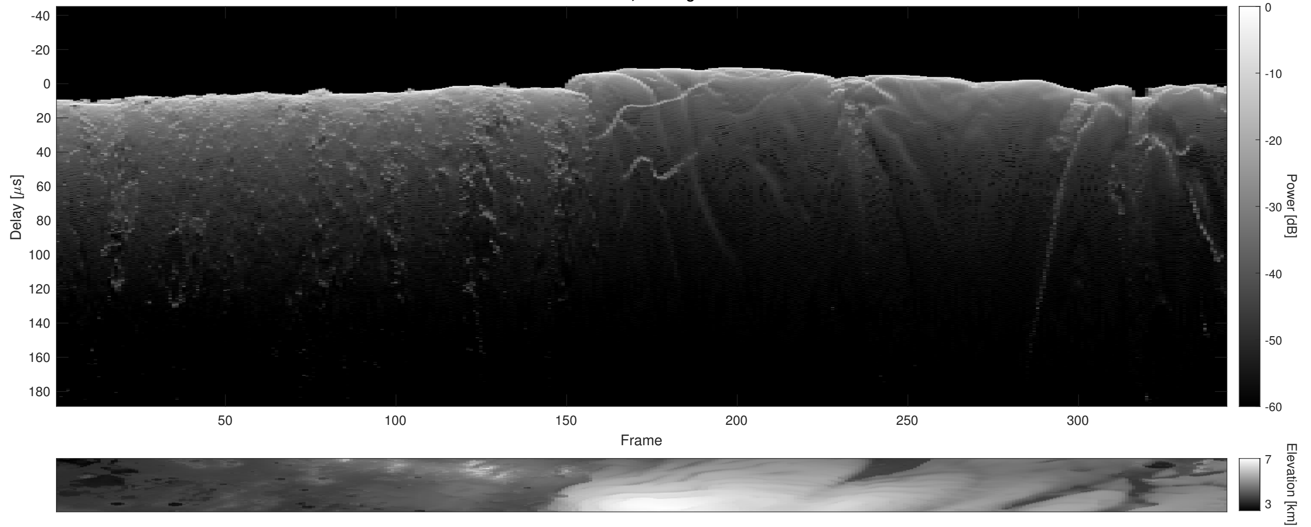
Orbit 4396, Cluttergram
