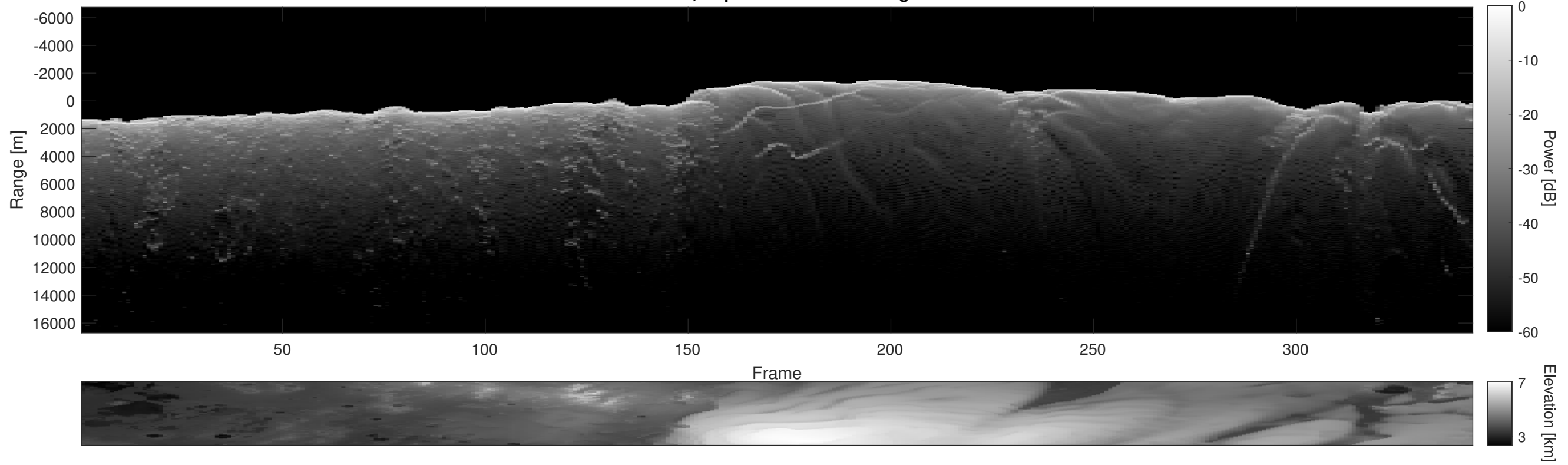
Orbit 4396, Depth-Corrected Cluttergram
