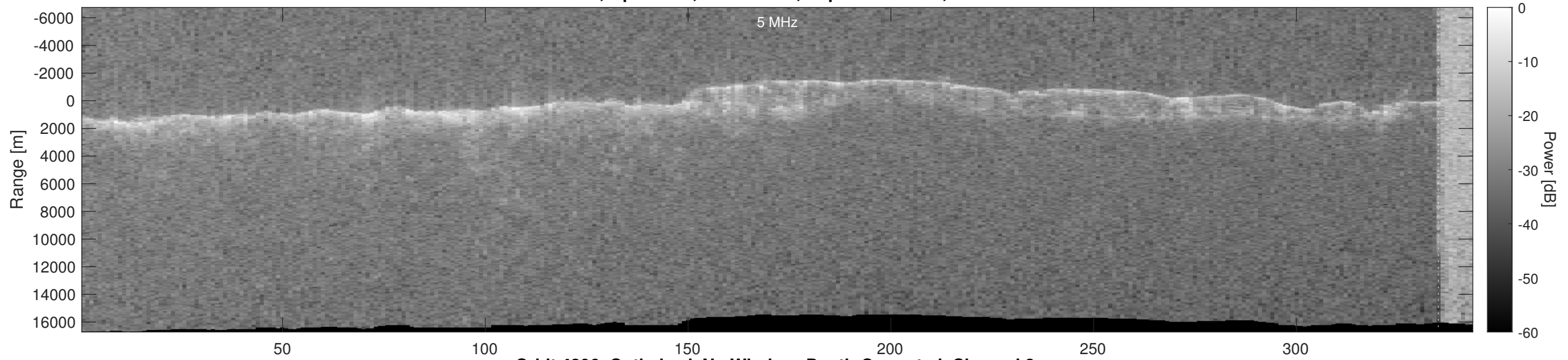
Orbit 4396, Optimized, No Window, Depth-Corrected, Channel 2
