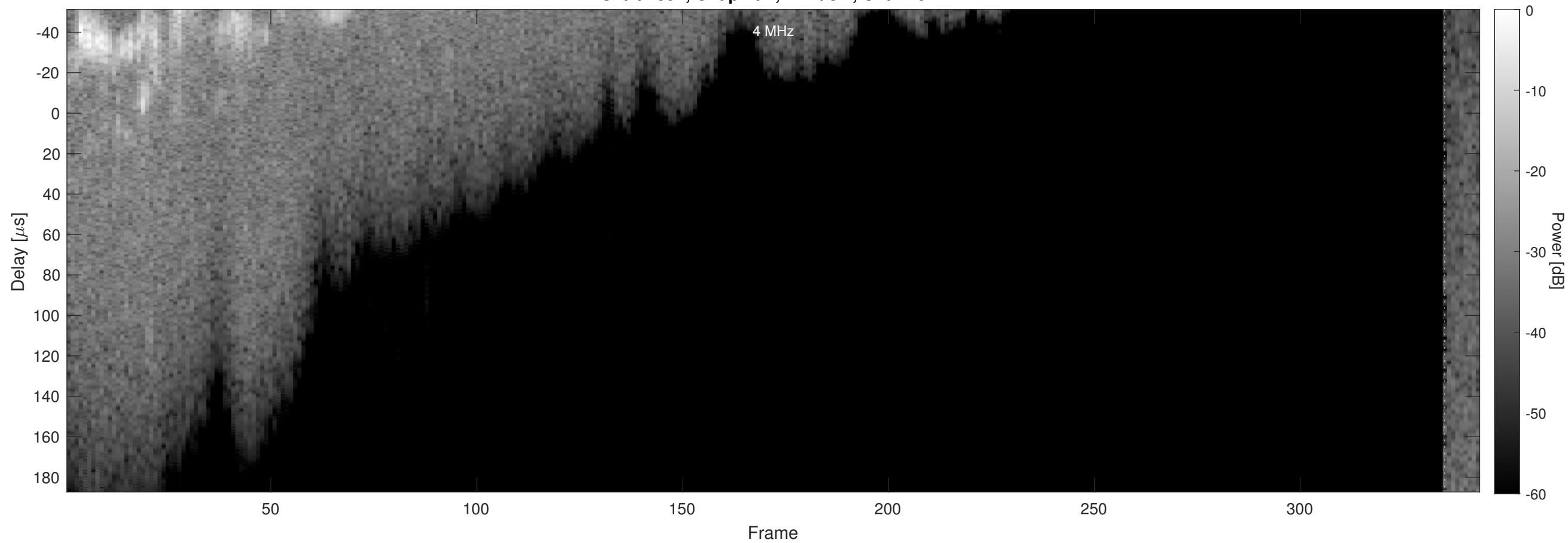
Orbit 4397, Chapman, Window, Channel 2
