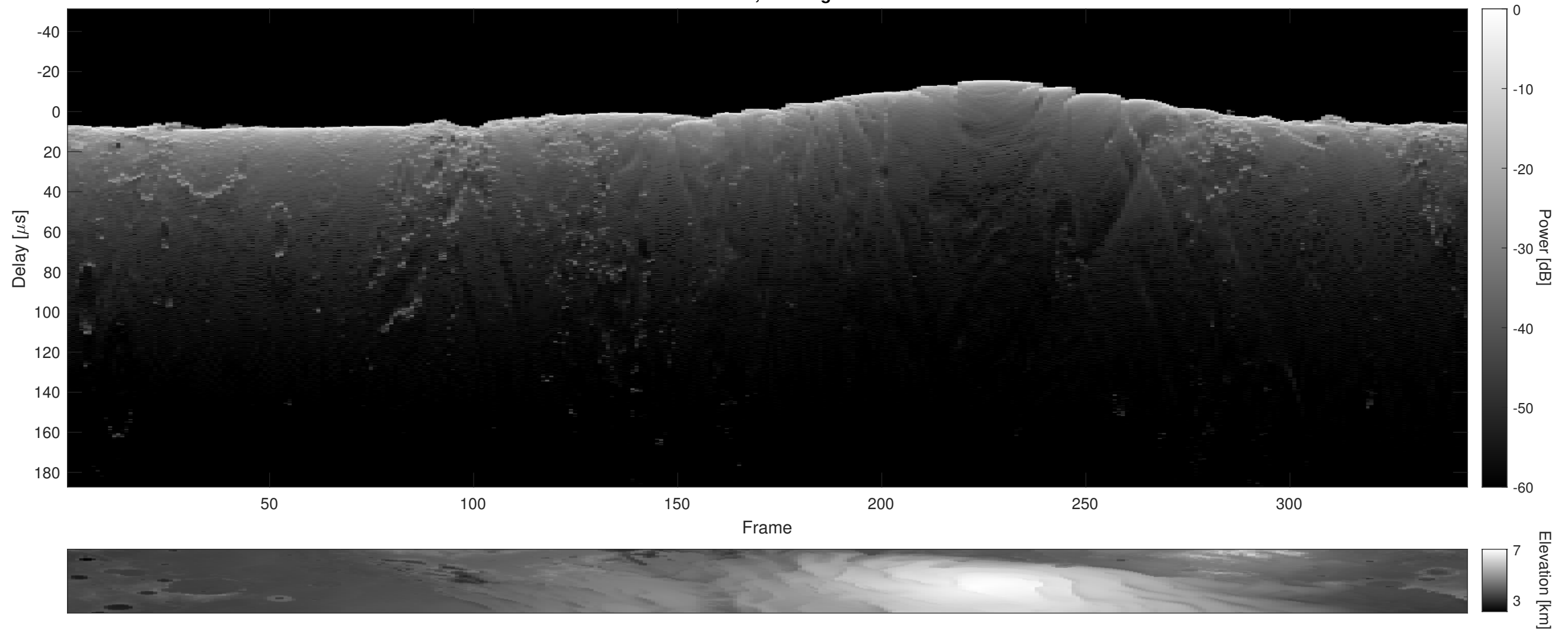
Orbit 4397, Cluttergram
