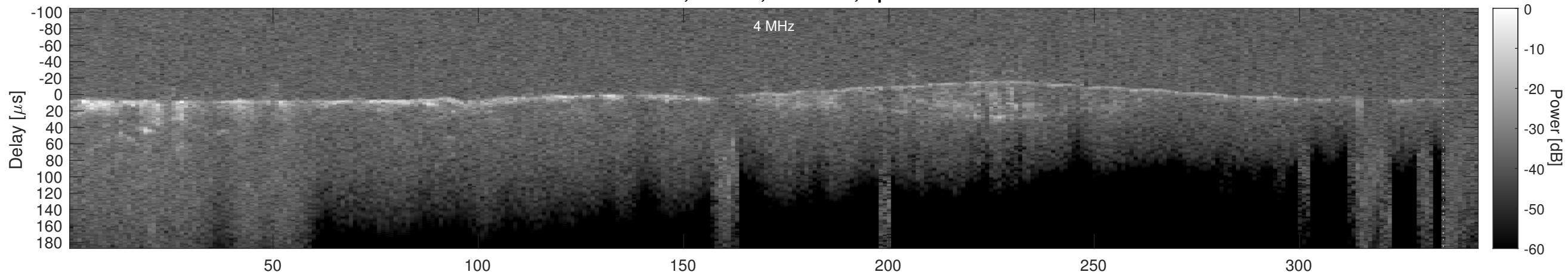
Orbit 4397, Cluttergram
