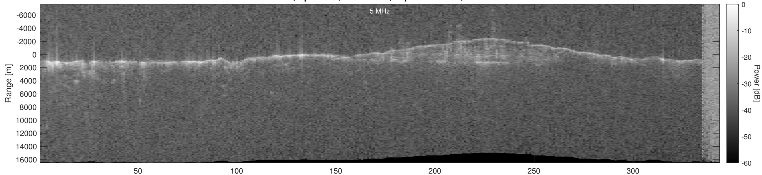
Orbit 4397, Optimized, No Window, Depth-Corrected, Channel 2
