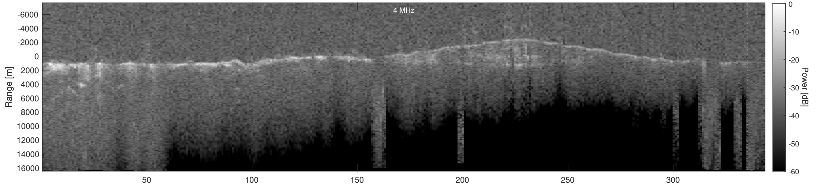
Orbit 4397, Depth-Corrected Cluttergram
