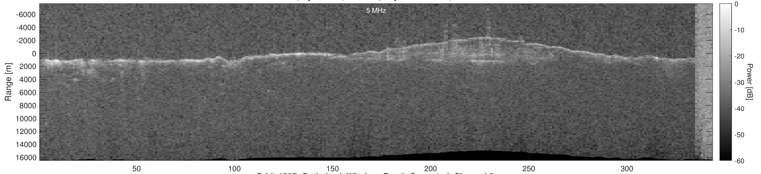
Orbit 4397, Optimized, Window, Depth-Corrected, Channel 2
