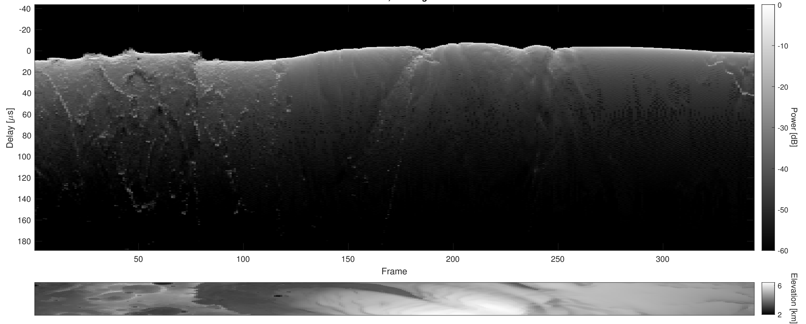
Orbit 4399, Cluttergram
