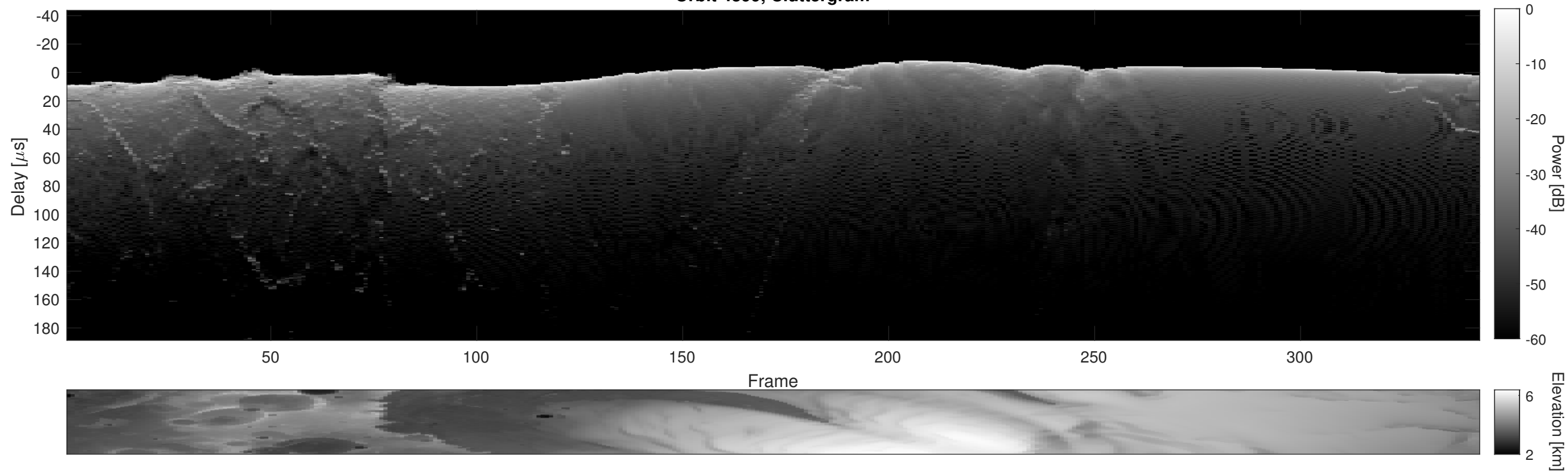
Orbit 4399, Cluttergram
