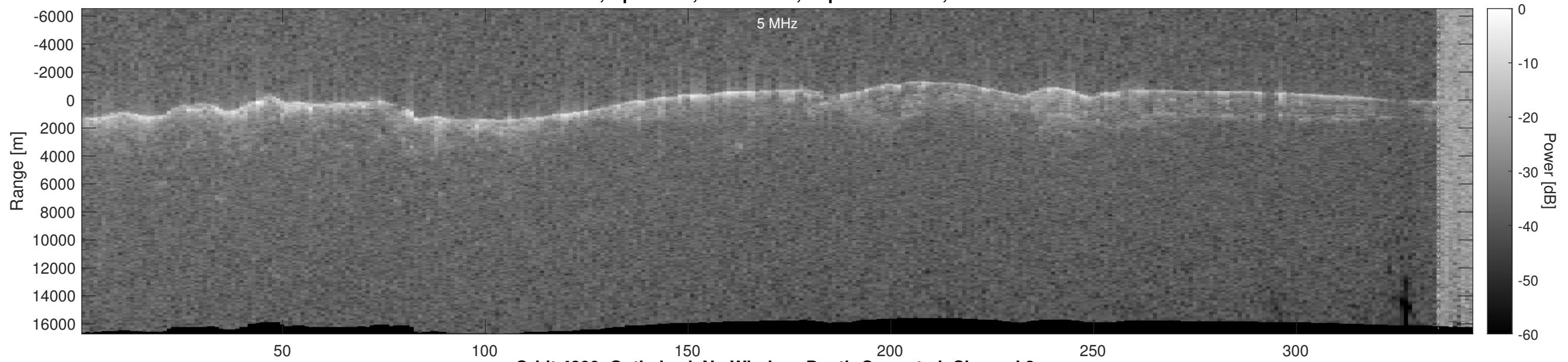
Orbit 4399, Optimized, No Window, Depth-Corrected, Channel 2
