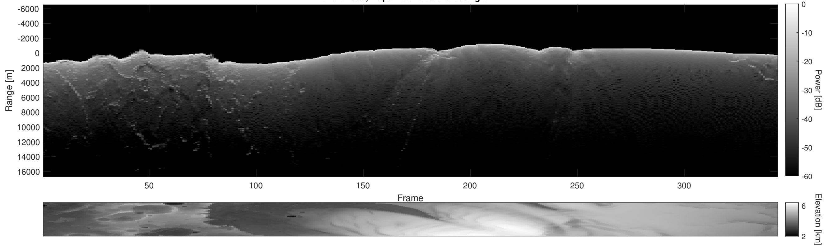
Orbit 4399, Depth-Corrected Cluttergram
