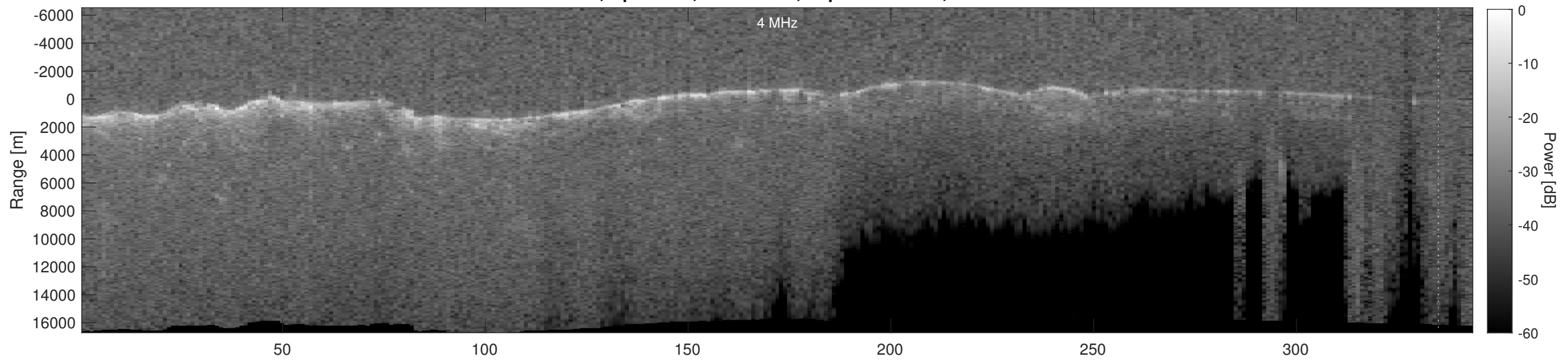
Orbit 4399, Depth-Corrected Cluttergram
