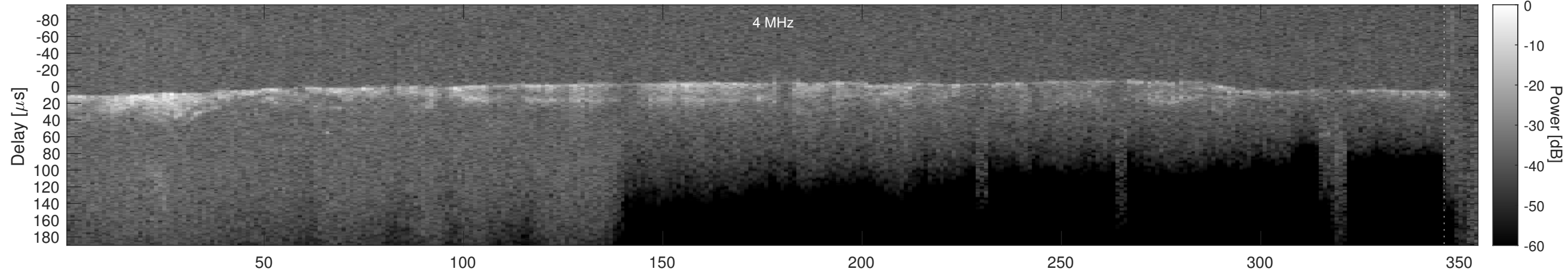
Orbit 4405, Cluttergram
