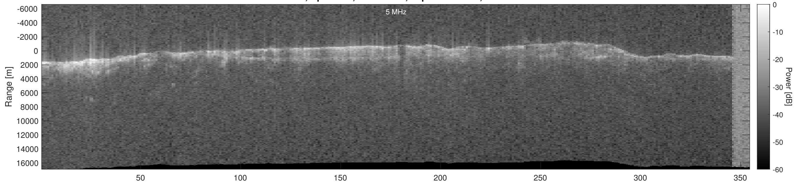
Orbit 4405, Optimized, No Window, Depth-Corrected, Channel 2
