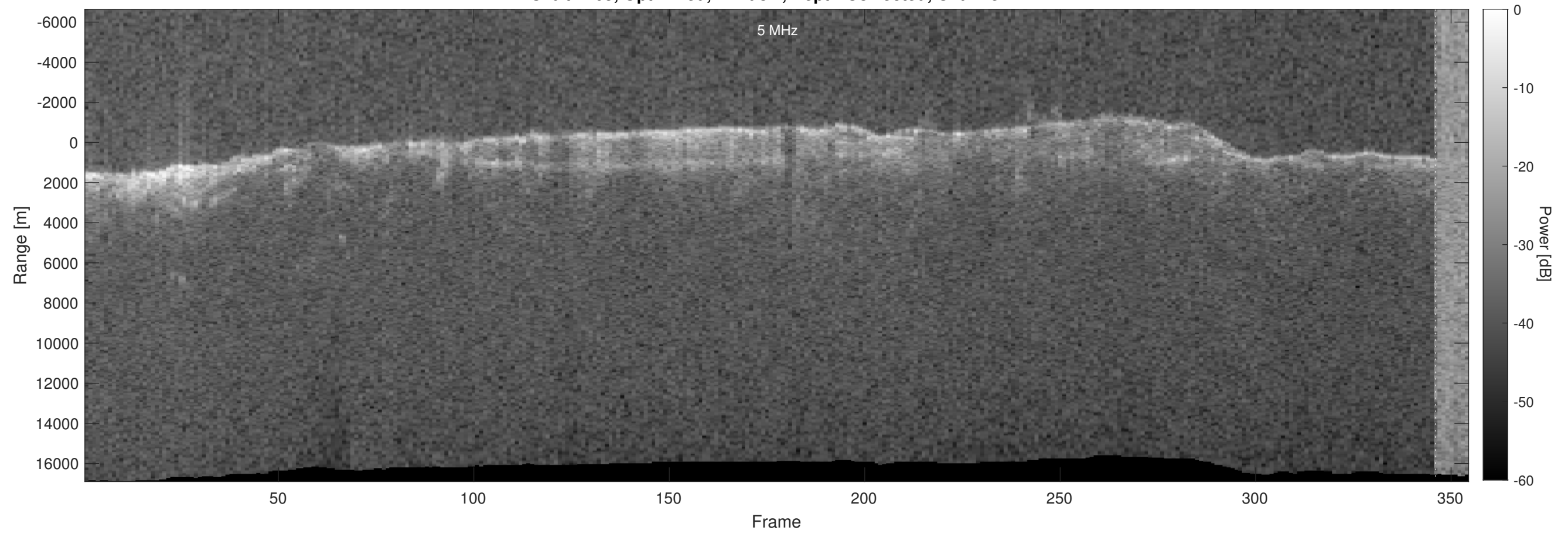
Orbit 4405, Optimized, Window, Depth-Corrected, Channel 2
