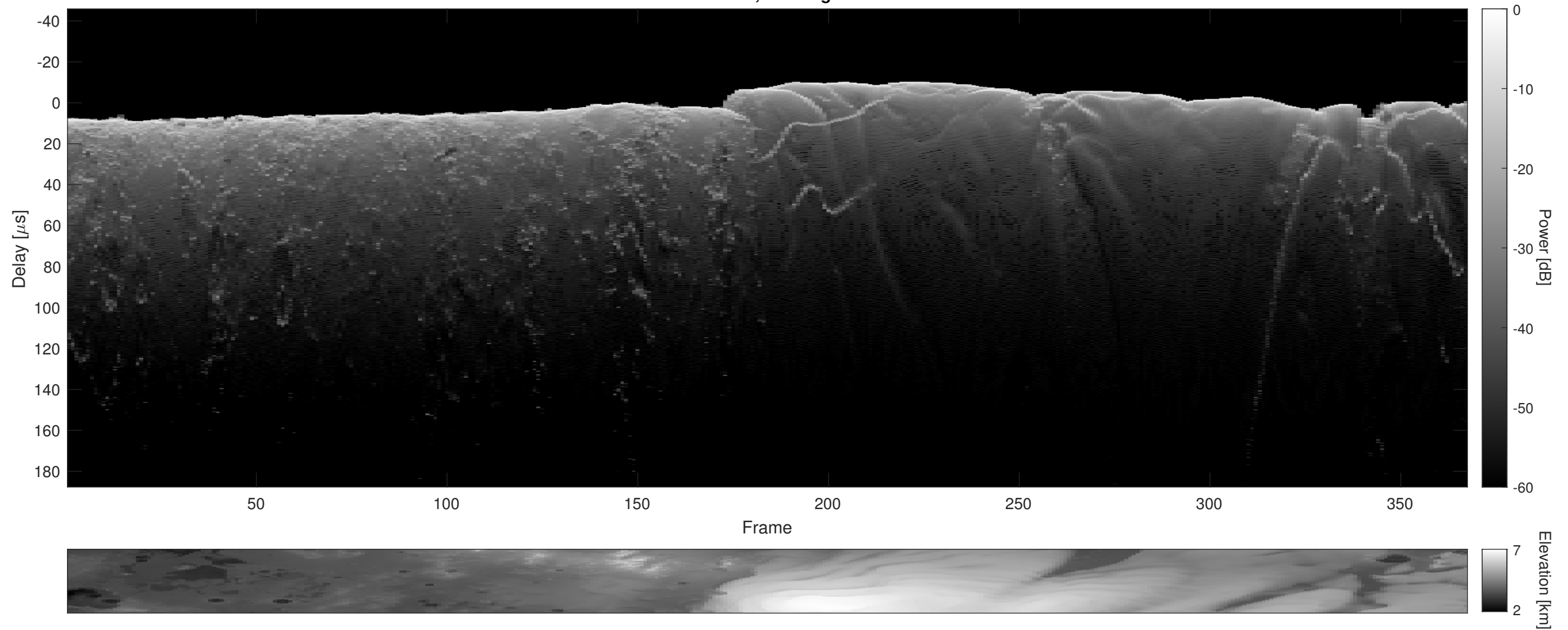
Orbit 4407, Cluttergram
