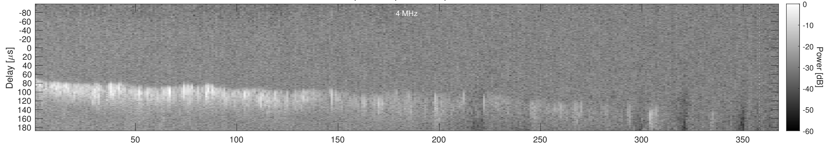
Orbit 4407, Window, Channel 2, Chapman
