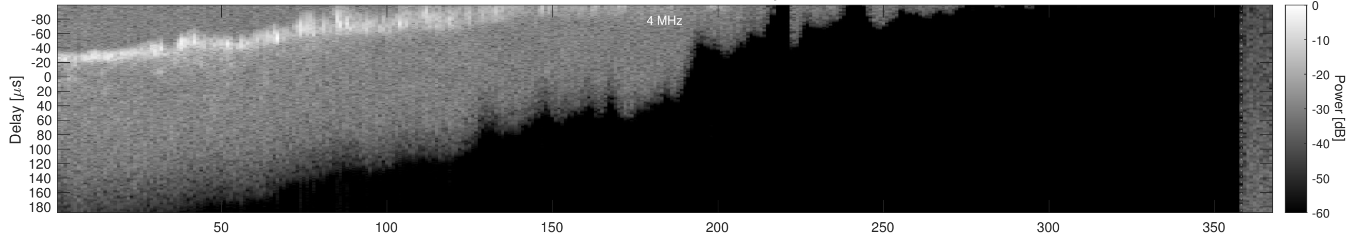
Orbit 4407, Window, Channel 2, Optimized
