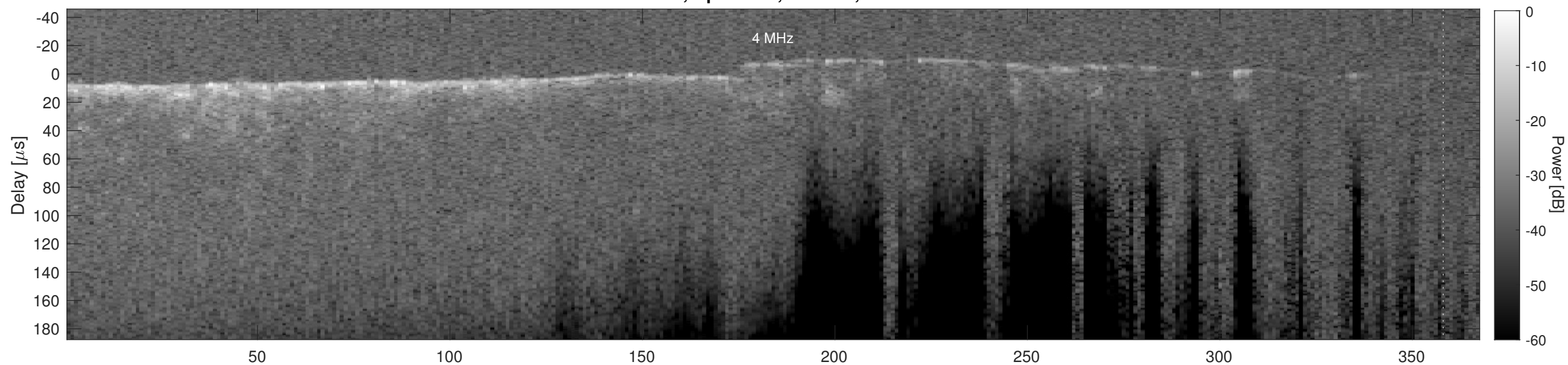
Orbit 4407, Cluttergram
