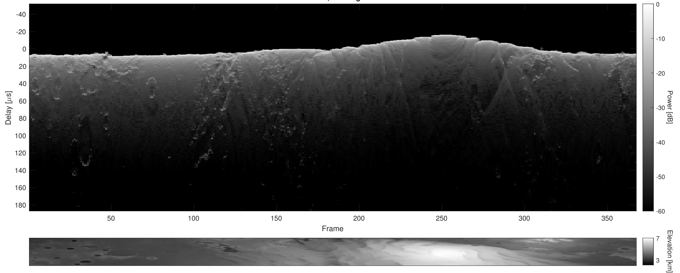
Orbit 4408, Cluttergram
