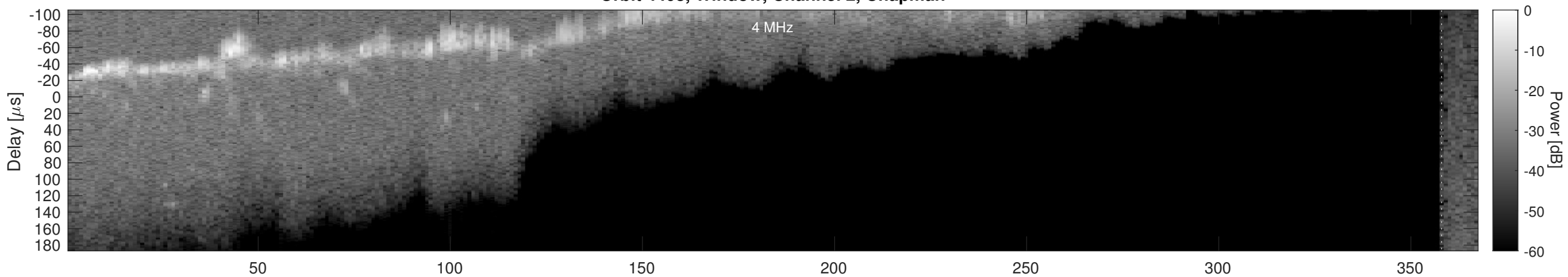
Orbit 4408, Window, Channel 2, Optimized
