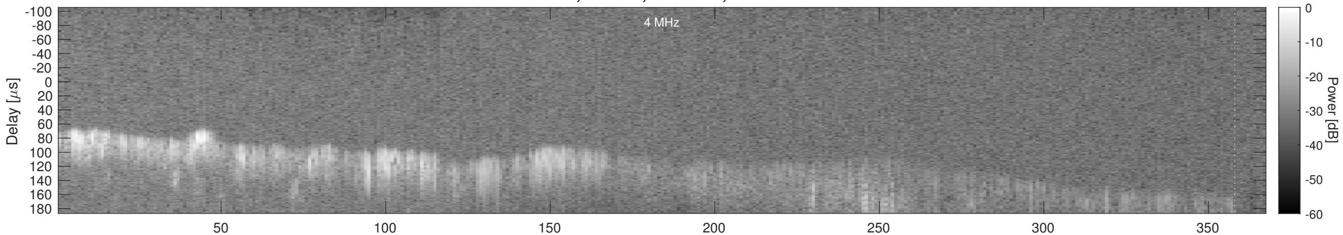
Orbit 4408, Window, Channel 2, Chapman
