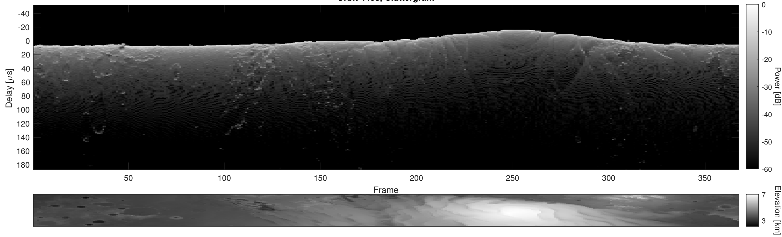
Orbit 4408, Cluttergram
