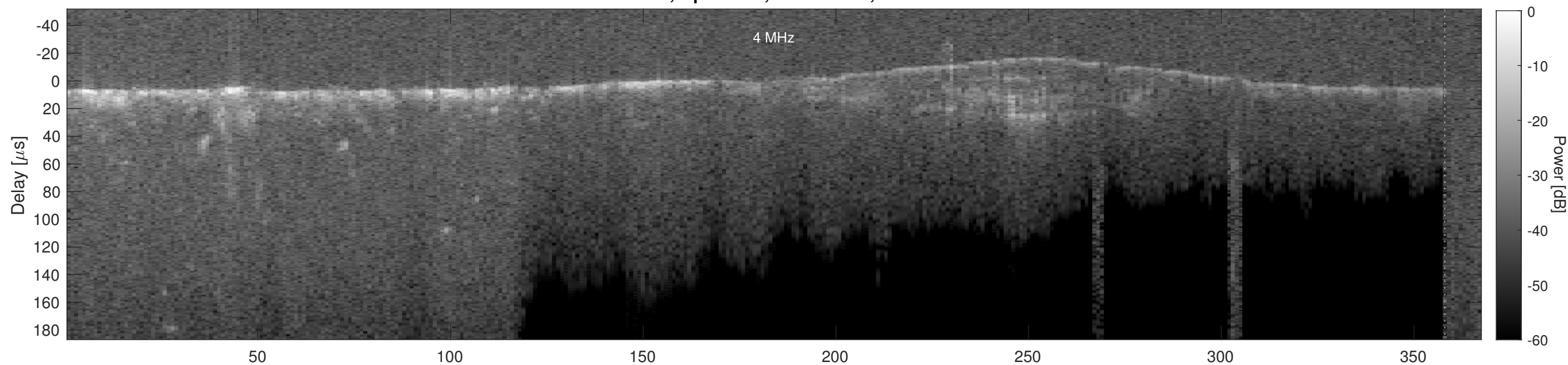
Orbit 4408, Cluttergram
