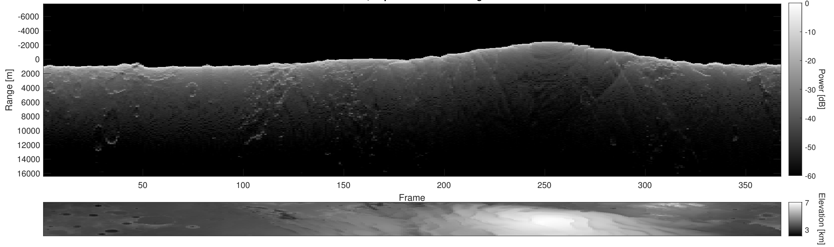
Orbit 4408, Depth-Corrected Cluttergram
