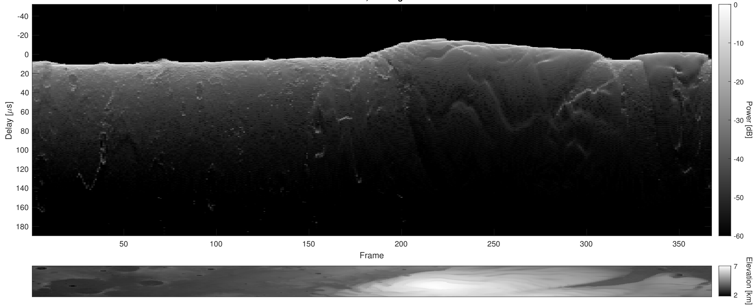
Orbit 4411, Cluttergram
