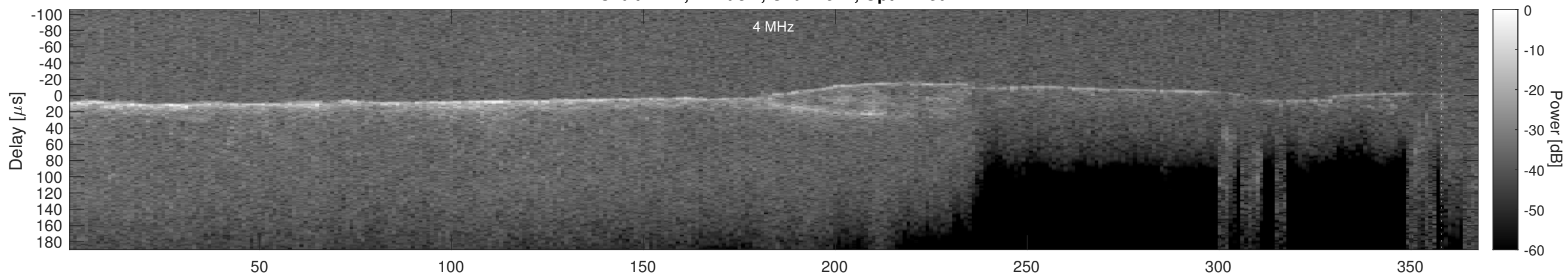
Orbit 4411, Cluttergram
