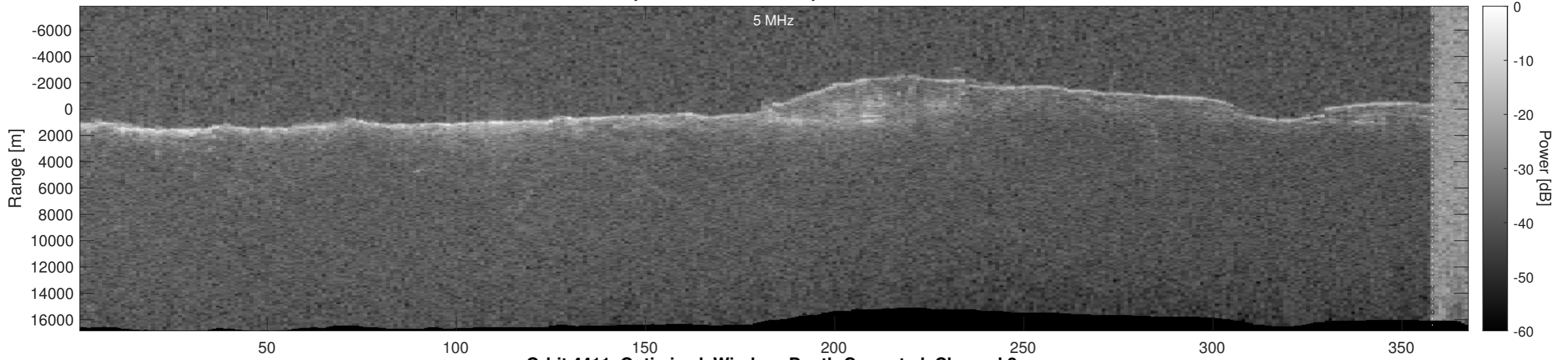
Orbit 4411, Optimized, Window, Depth-Corrected, Channel 2
