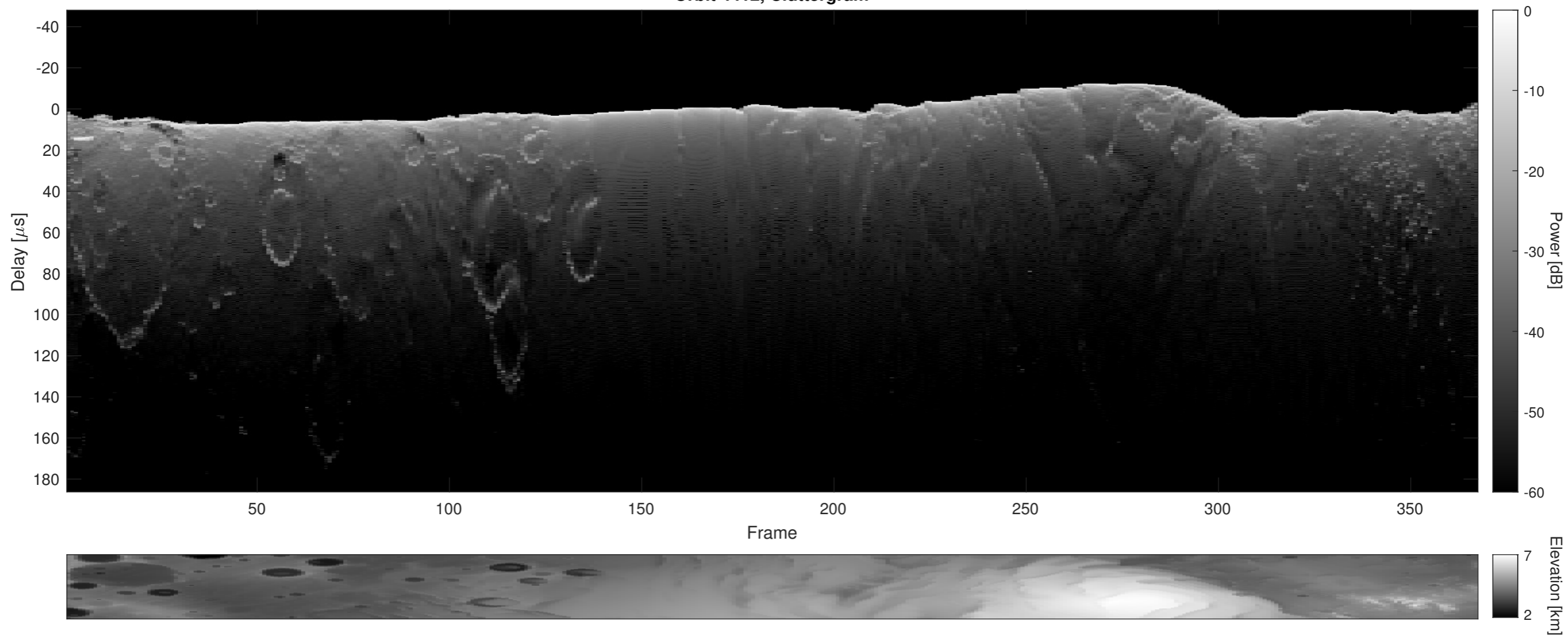
Orbit 4412, Cluttergram
