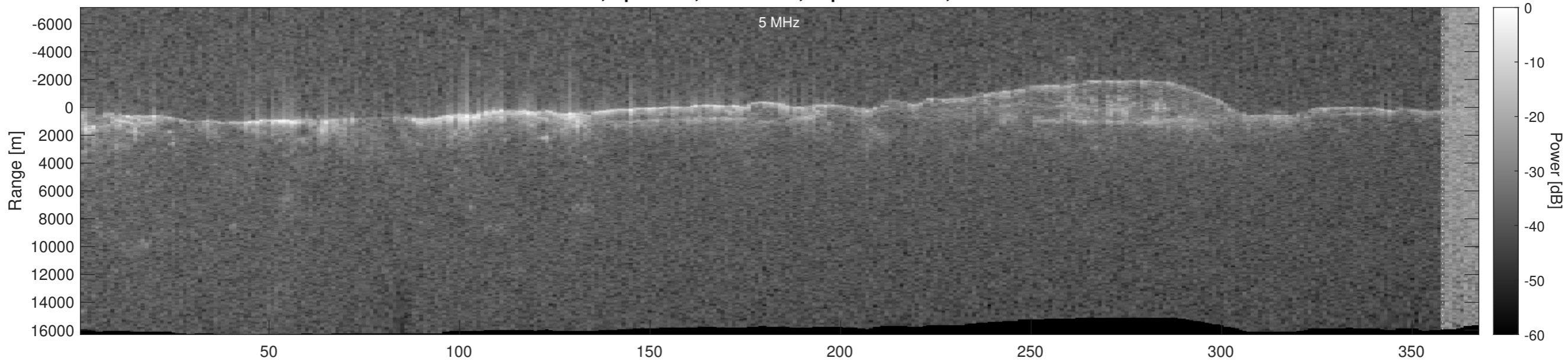
Orbit 4412, Optimized, No Window, Depth-Corrected, Channel 2
