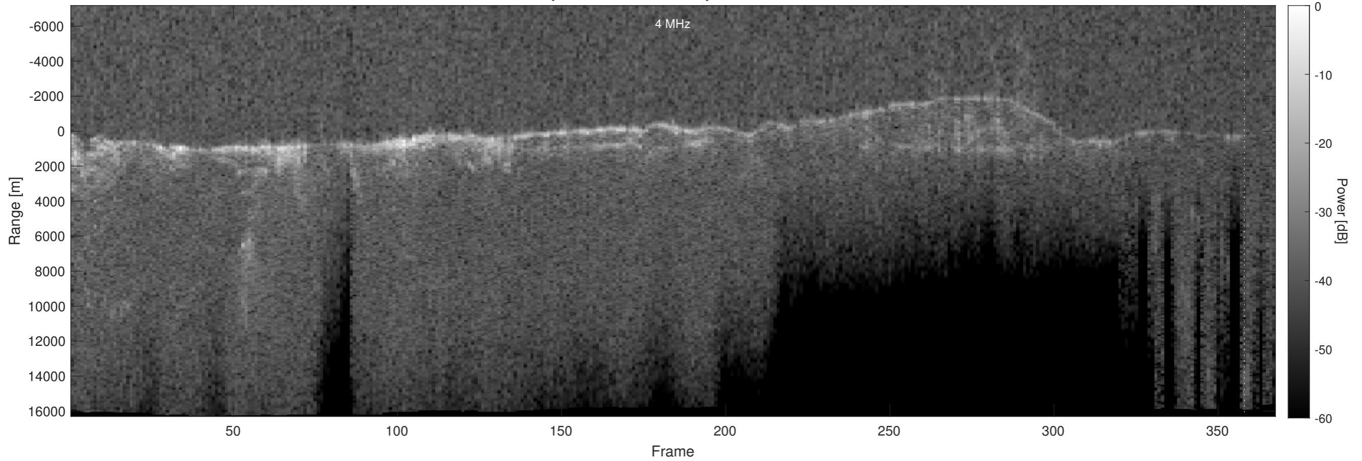
Orbit 4412, Optimized, Window, Depth-Corrected, Channel 2
