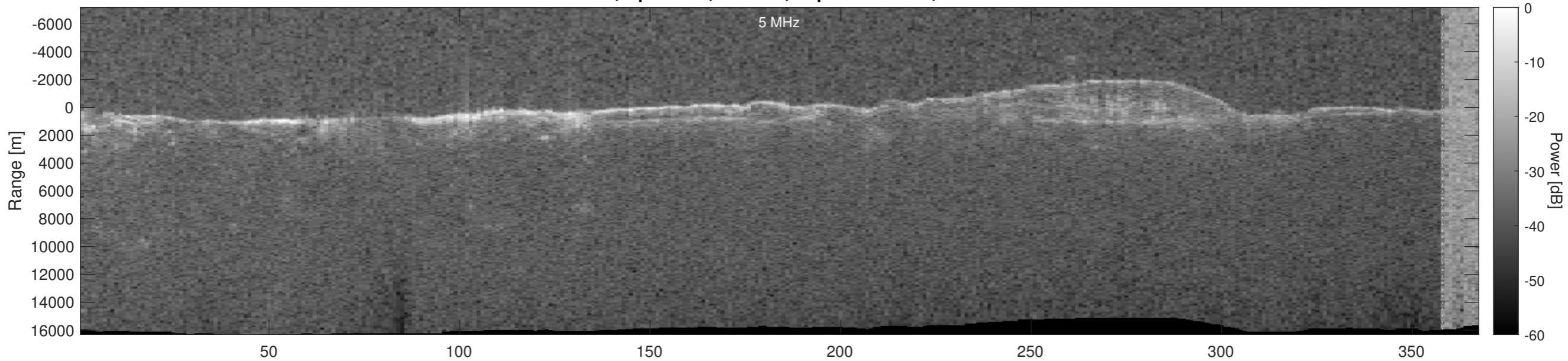
Orbit 4412, Optimized, Window, Depth-Corrected, Channel 2
