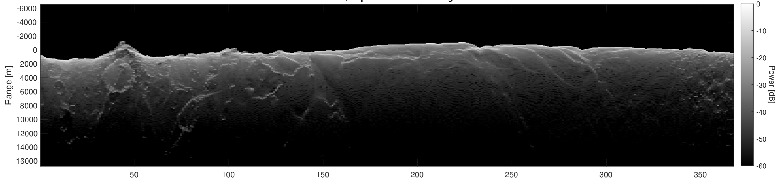
Orbit 4413, Depth-Corrected Cluttergram
