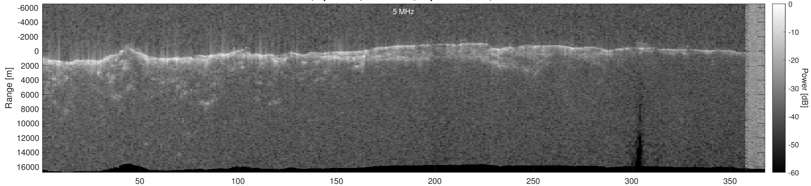
Orbit 4413, Optimized, No Window, Depth-Corrected, Channel 2
