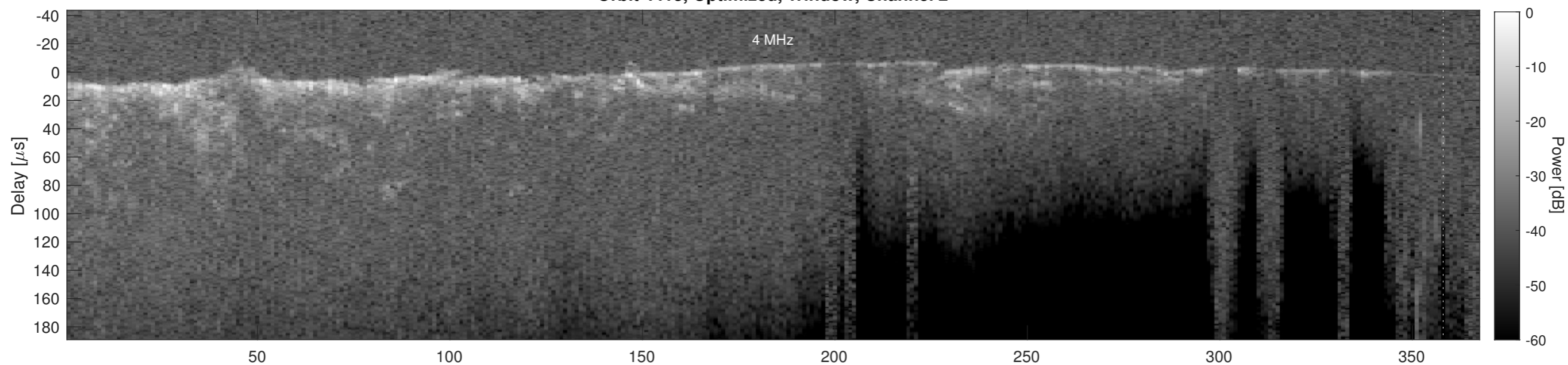
Orbit 4413, Cluttergram
