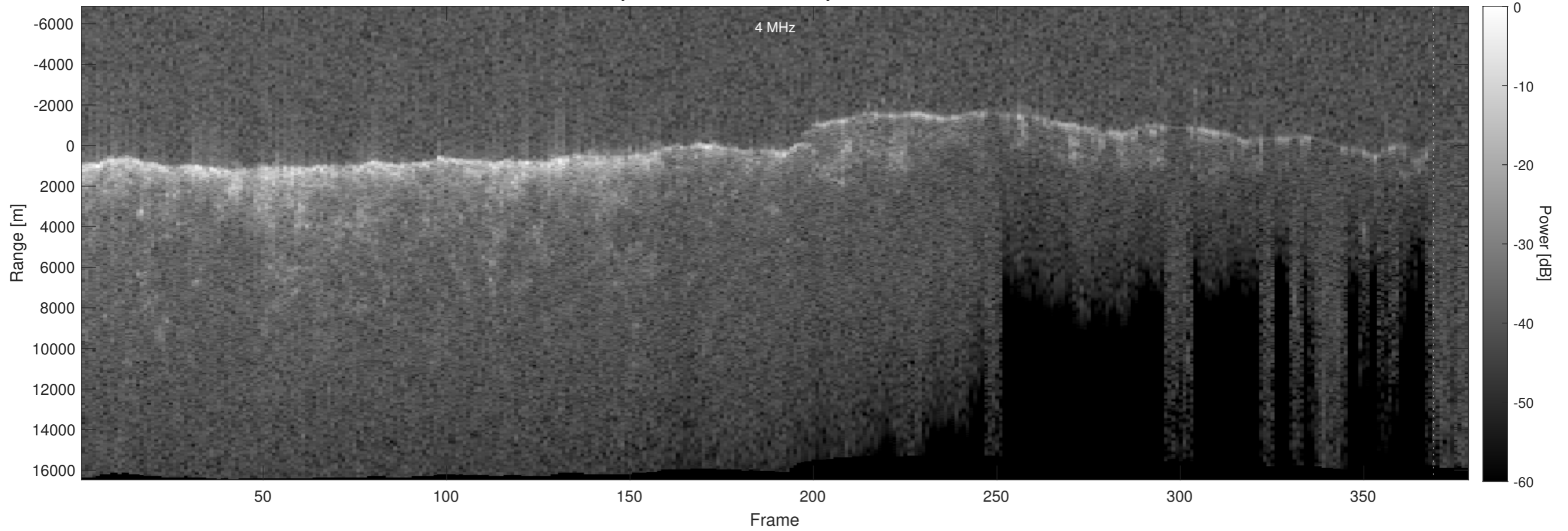
Orbit 4418, Optimized, No Window, Depth-Corrected, Channel 2
