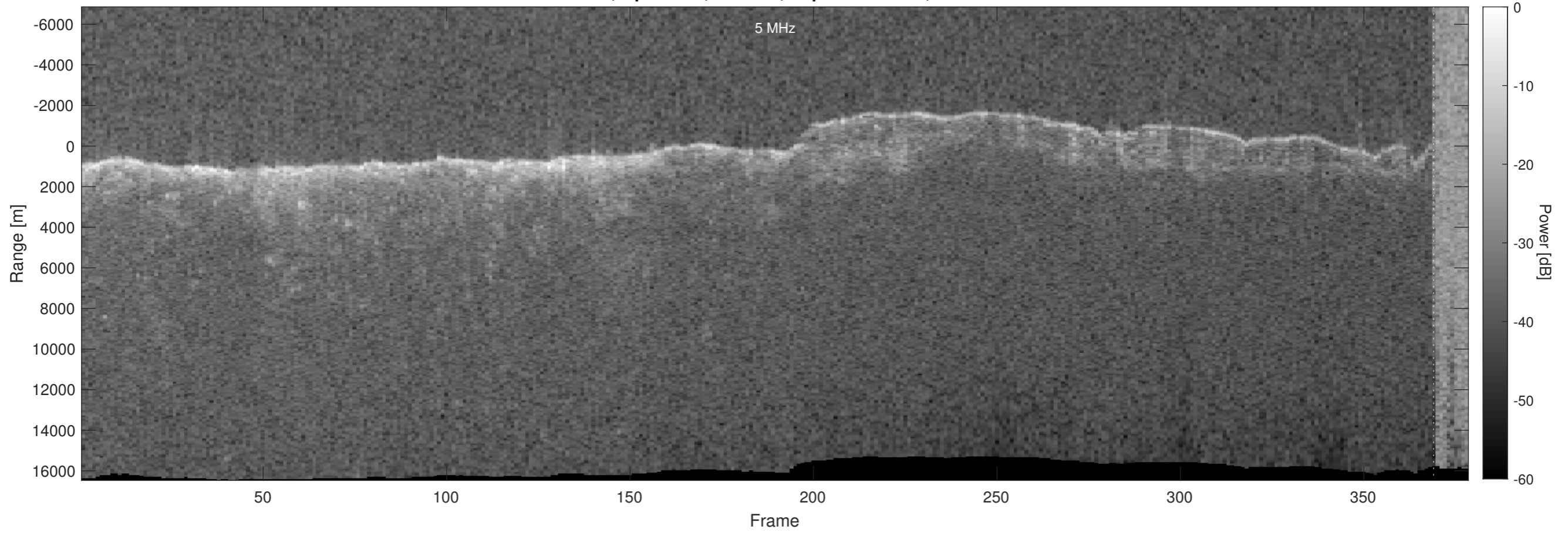
Orbit 4418, Optimized, Window, Depth-Corrected, Channel 2
