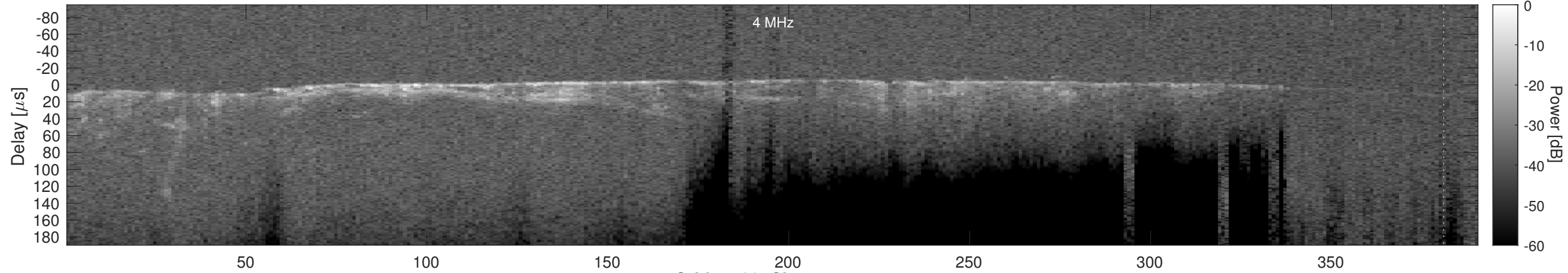
Orbit 4420, Cluttergram
