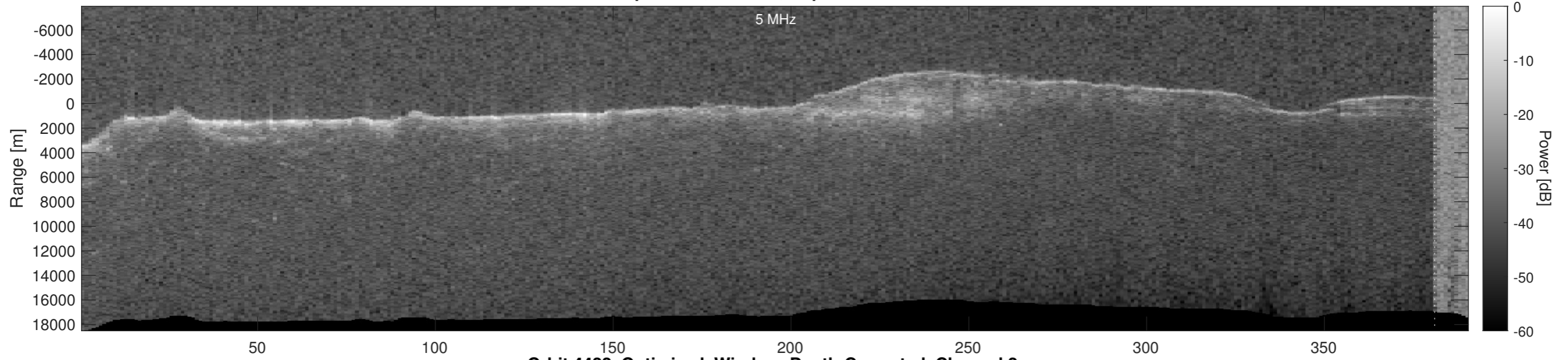
Orbit 4422, Optimized, Window, Depth-Corrected, Channel 2
