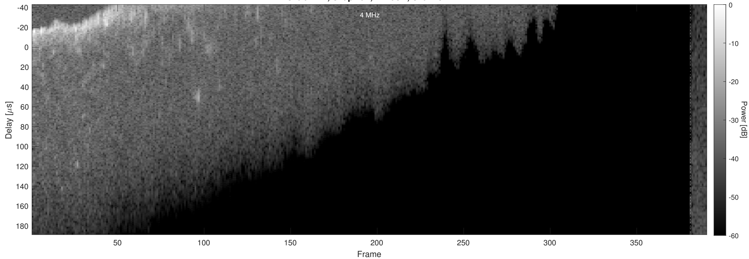
Orbit 4424, Chapman, Window, Channel 2
