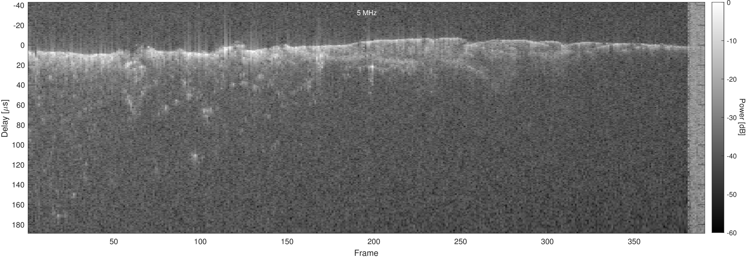
Orbit 4424, Optimized, No Window, Channel 2
