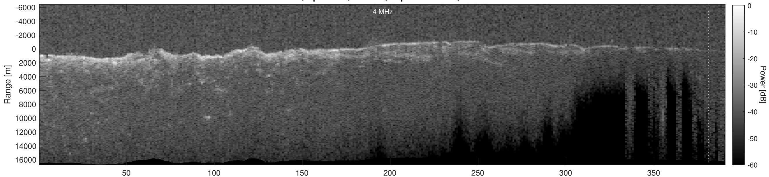
Orbit 4424, Depth-Corrected Cluttergram
